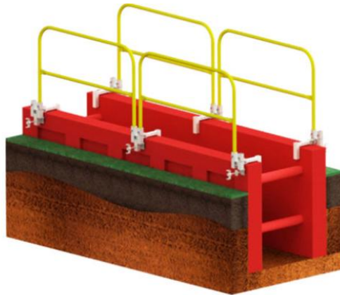
Trench Box Clamp-on Guardrail System www.garlocksafety.com
